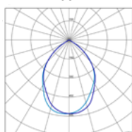
ATEX LED MAX 190W 65°
