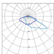
ATEX LED MAX 190W ASYMM
